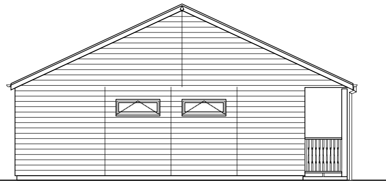
Left Elevation
